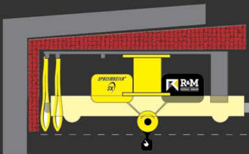
Figure 1. C-track Festoon
